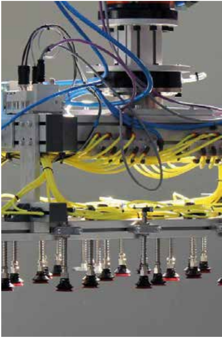
END-OF-ARM-TOOLING (EOAT)
